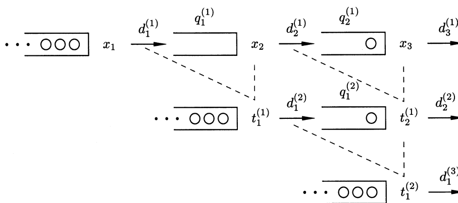
FIGURE 1. The series of queues in series ( k = 3 )
