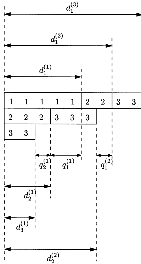
FIGURE 2. The tableau \tau(17)
